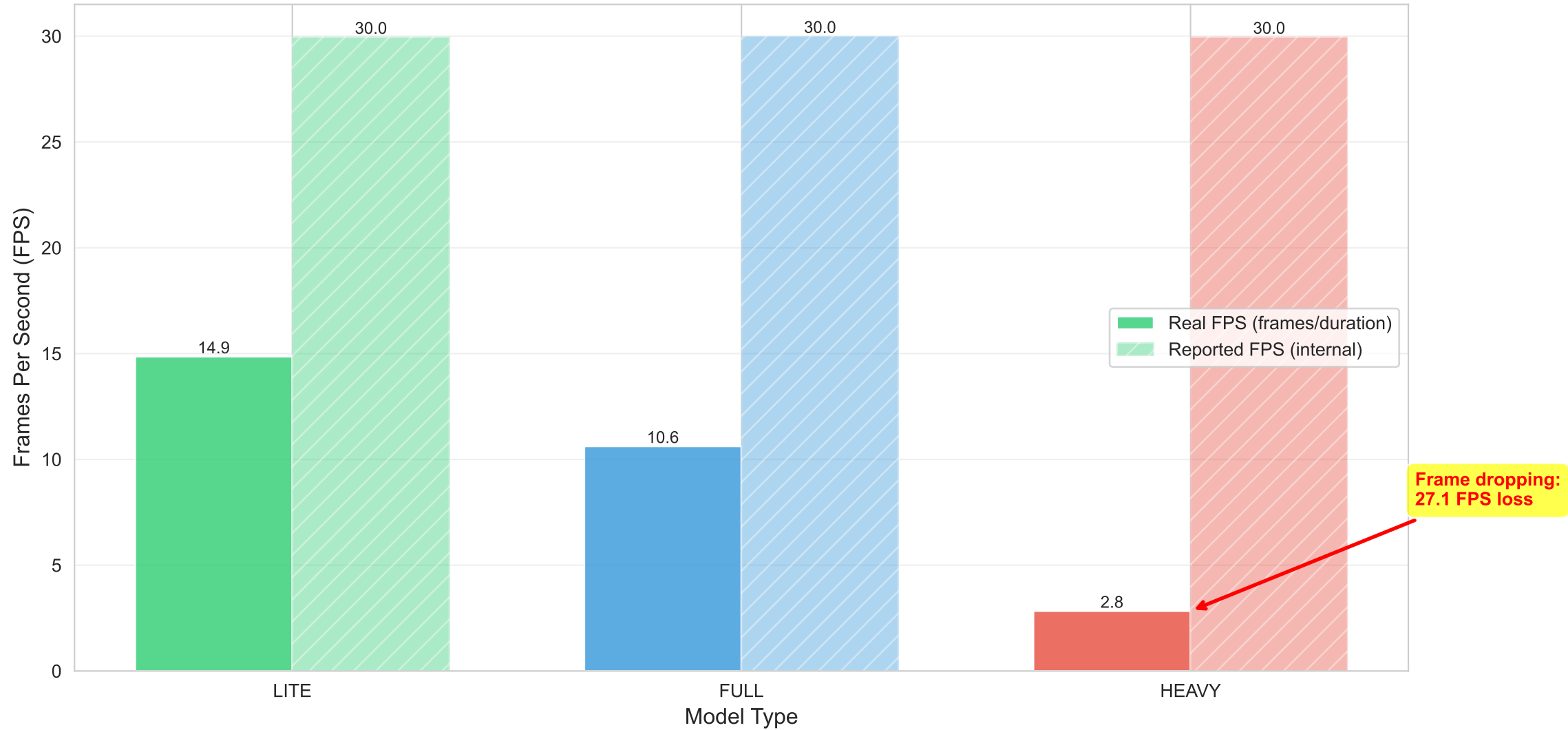
Real FPS vs Reported FPS - Frame Dropping Analysis
